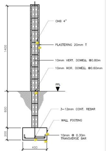
S1 02 WALL FOOTING AND CHB LAYOUT PLAN SCALE: 1:16 mm
