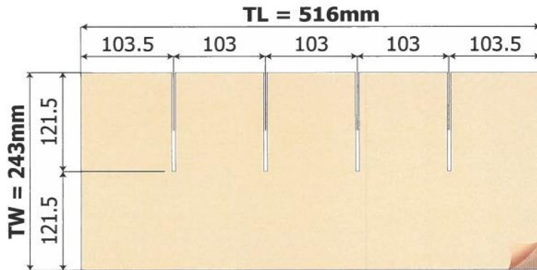
PARTITION LONG 1PC.
