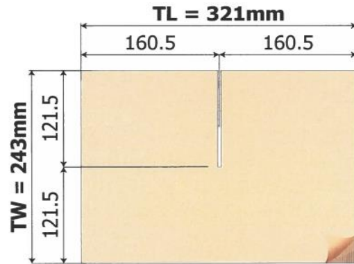
PARTITION SHORT 4PCS.
